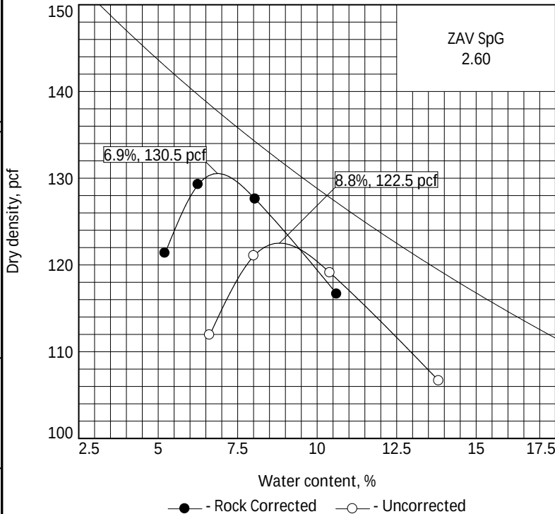
COMPACTION TESTING DATA ASTM D 1557-12 Method C Modified ASTM D4718-15 Oversize Corr. Applied to Each Test Point
